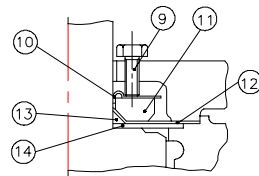
ENLARGED VIEW OF TOP SEAL
